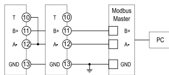
RS485 Modbus communication port
